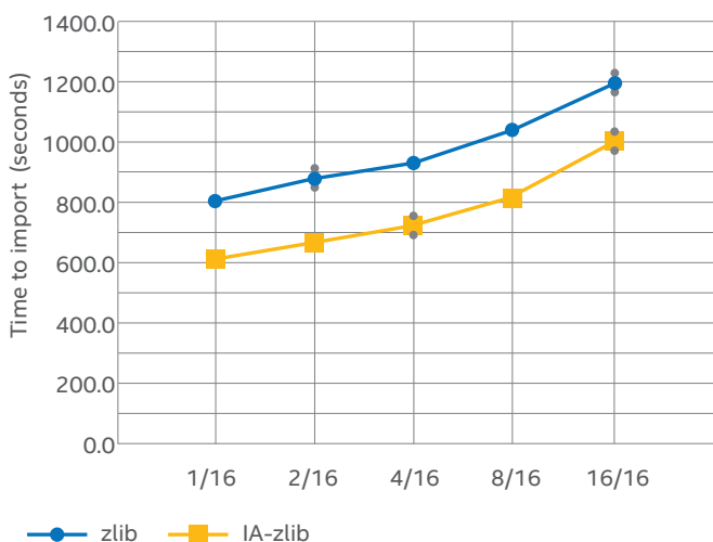
Figure 8. Comparison of import times of 1, 2, 4, 8, and 16 partitions of human genome from 1,000 samples with standard zlib and compression libraries optimized for Intel® architecture.
