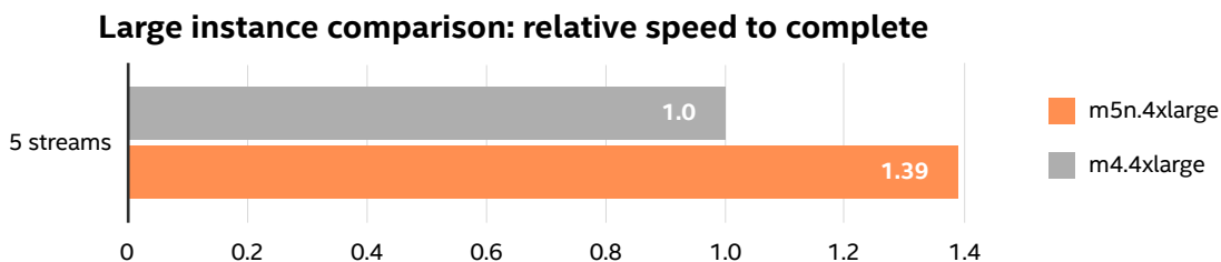
Figure 2. Relative speed to complete multiple query streams from a TPC-H-like HammerDB workload running against Microsoft SQL Server databases on large-sized instances.
