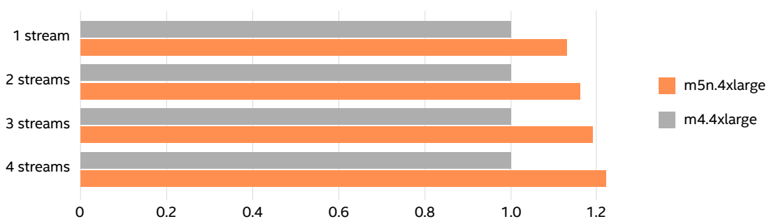
Figure 1. Relative speed to complete multiple query streams from a TPC-H-like HammerDB workload running against Microsoft SQL Server databases on medium-sized instances.
