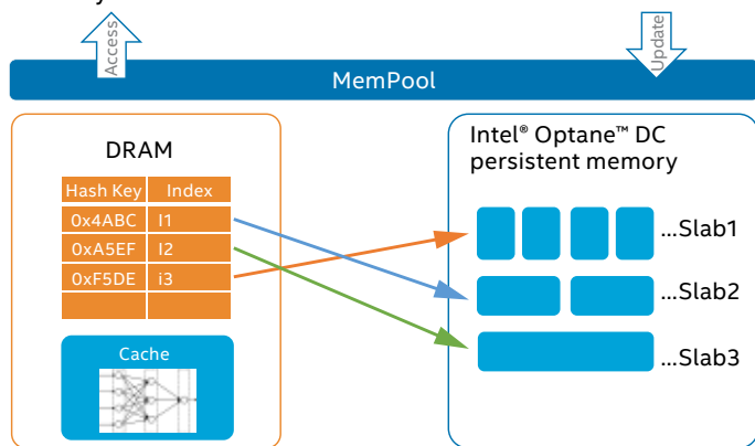
Fig. 3 Heterogeneous storage system built on Intel® Optane™ DC persistent memory
