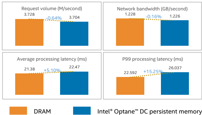
Fig. 4 Pressure test results of the indexing system based on Intel® Optane™ DC persistent memory
