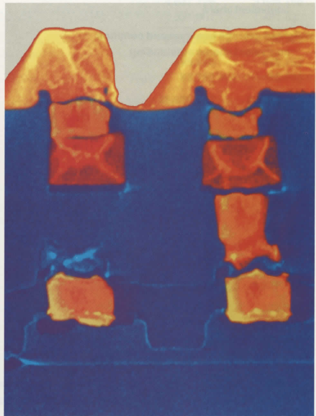
This magnified cross-section of a wafer, manufactured on Intel's three-layer metal logic process technology, reveals the minute structural detail of a chip. Thanks to this advanced interconnect technology, lines less than \frac{1}{1000} th the thickness of a human hair can be squeezed onto a small surface area to make Intel's fastest, most powerful processors.
